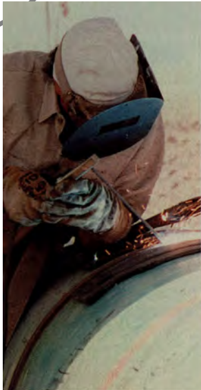
A welder makes a hot pass on a section of pipe.
