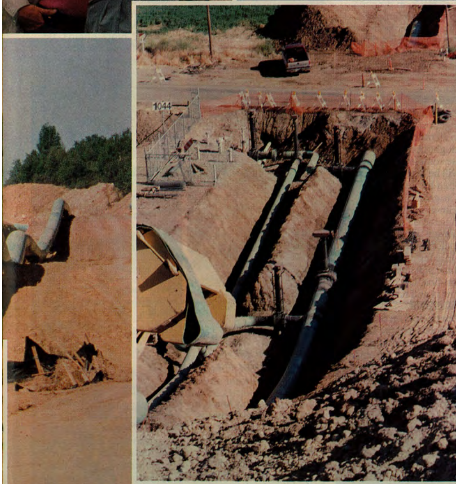
In this photograph, the pipe gang and hot pass filler crew are working on the San Joaquin Valley portion of the pipeline, which flows through the hills and fertile fields of this productive valley.
